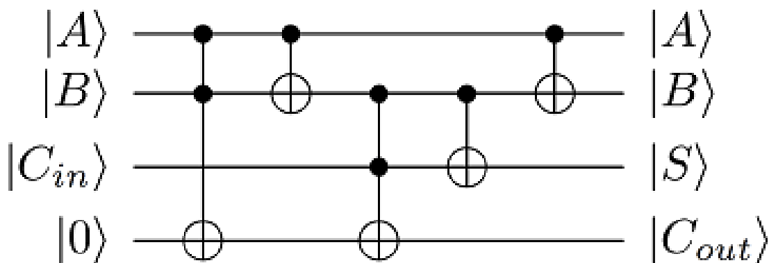
Figure 2: Full Quantum Adder (with carry)
